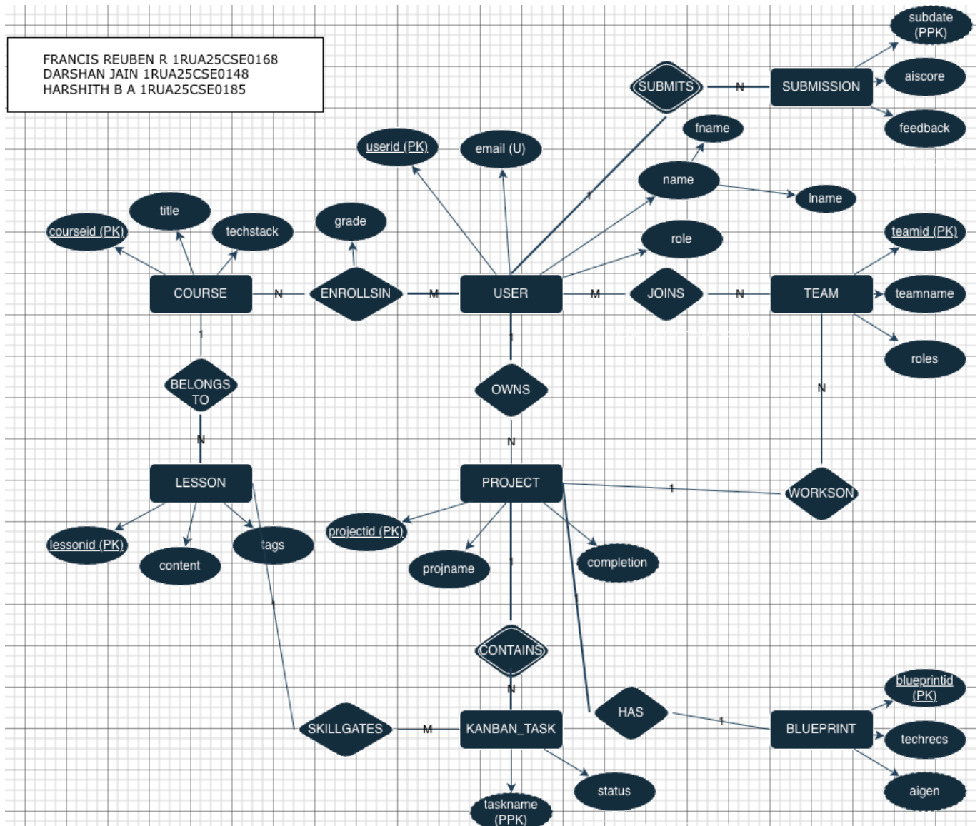
Figure 1: DevPath ER Diagram
